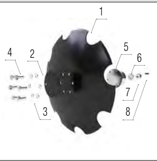
Disc zimțat 520 × 5 mm
