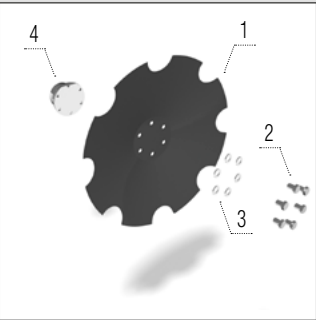
Disc zimțat 460 × 5 mm
