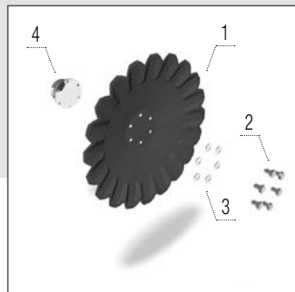
A-Disc 520 × 5 mm
