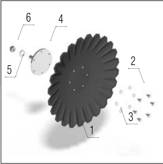
A-Disc 620 × 6 mm
