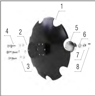
Disc zimțat 560 x 5 mm
