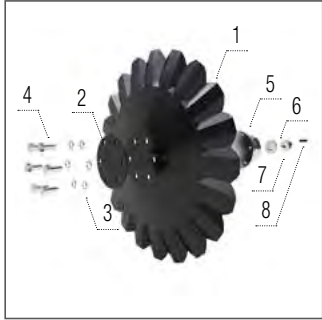
A-Disc 560 × 5 mm
