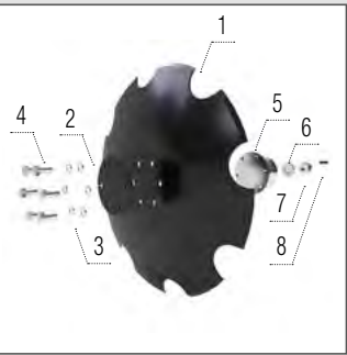
Disc zimțat 560 × 5 mm
