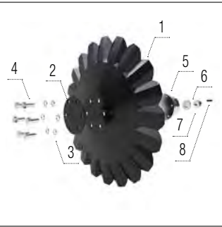
A-Disc 560 × 5 mm
