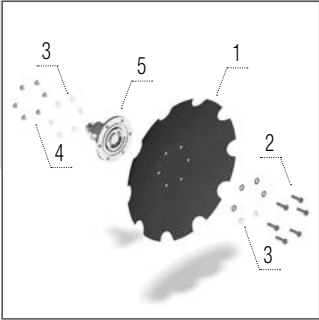
Disc zimțat 660 × 6 mm
