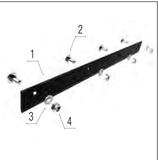
Trash Cutter 750
