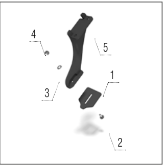
Cutpack sárkaparó
