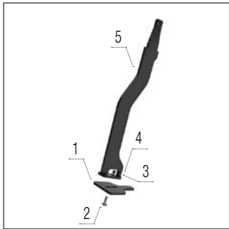
Cutpack sárkaparó
