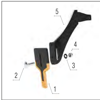
Hardface Cutpack sárkaparó
