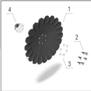
Disque A (agressif) 460 × 5 mm
