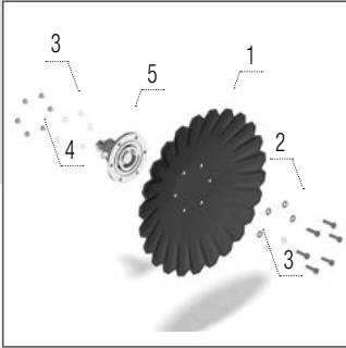
Disque A (agressif) 660 × 6 mm
