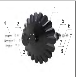
Disque A (agressif) 560 × 5 mm
