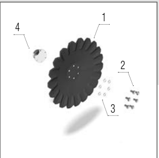
Disque A (agressif) 520 x 5 mm
