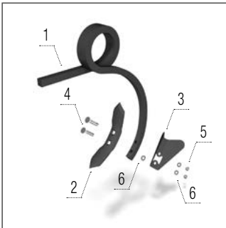
Pointe 60 mm
