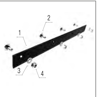
Trash Cutter 750
