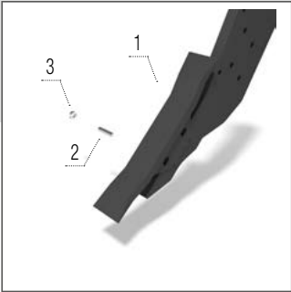
Pointe 70 mm
