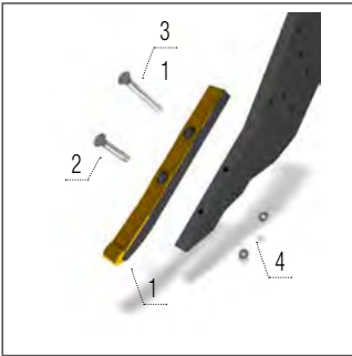
Pointe 40 mm LONG LIFE
