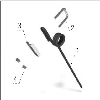
Harrow tine 10 mm
