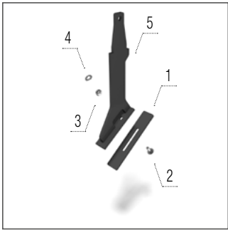
V-Ring roller scraper
