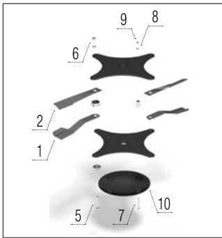
Corn blades – left + rotor cover
