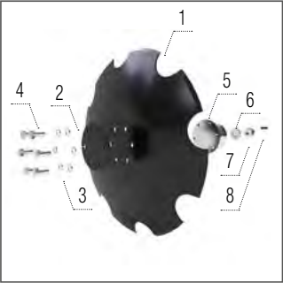
Serrated disc 560 × 5 mm
