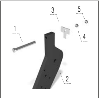
Tension bolt D
