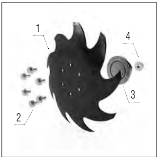
9-LH Star
