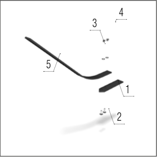
Spring roller scraper
