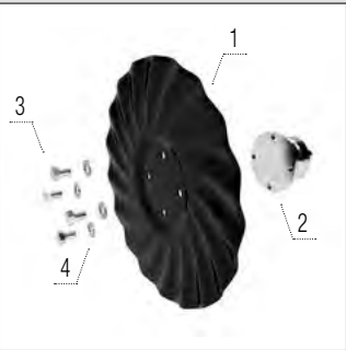
Left turbo coulter
