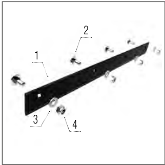
Trash Cutter 750
