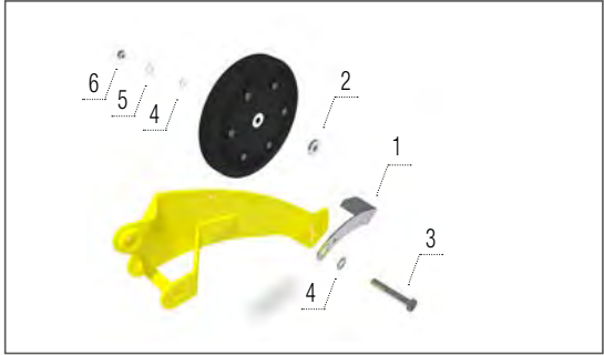
Classic depth wheel scraper
