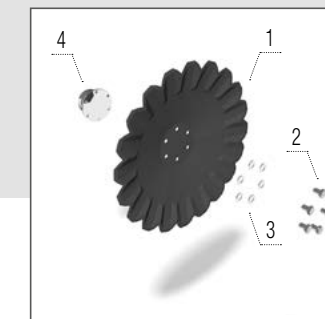
A-disc 520 × 5 mm
