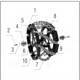
Chain roller 200
