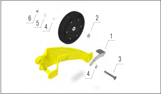
Hardface depth wheel scraper
