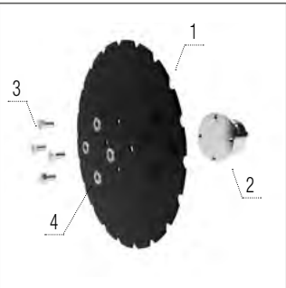
Fertilizing coulter
