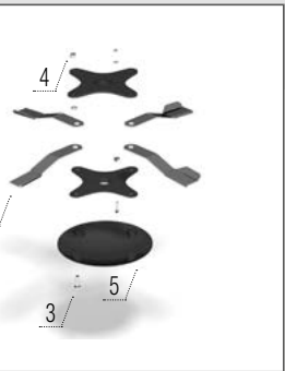
Grass blades – right + rotor cover
