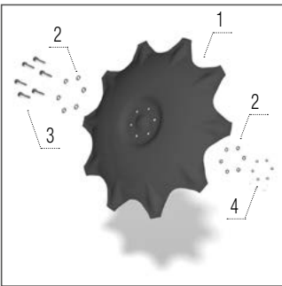
Protective disc
