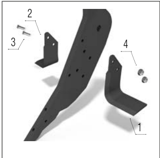
Left and right wing
