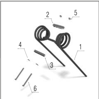
Tine
