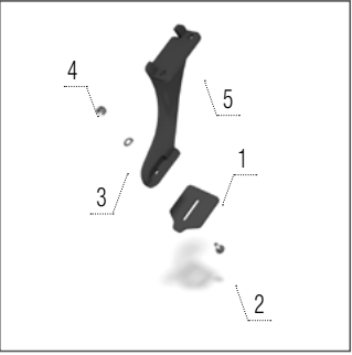
Cutpack scraper
