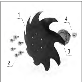
9-RH Star
