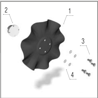
Coulter
