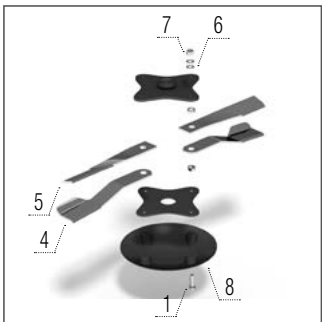
Corn blades – right + rotor cover
