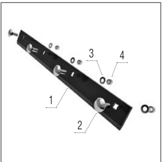
Trash Cutter 610
