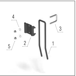
Harrow tine in front of double roller
