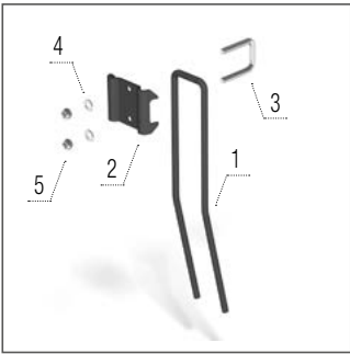
Front harrow tine
