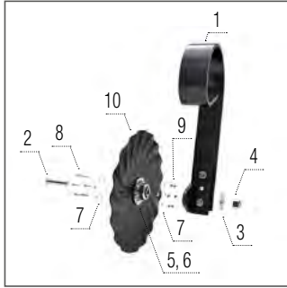
Coulter – right
