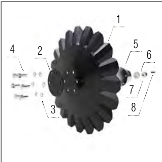
A-disc 560 × 5 mm
