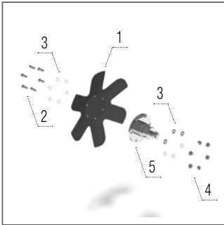
Levelling star disc – right
