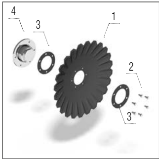
A-disc for the central unit 620 × 6 mm
