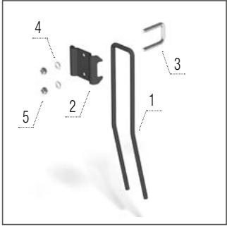
Harrow tine after single roller
