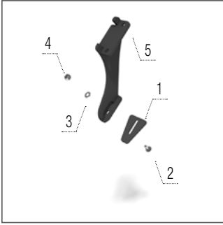
Rubberpacker scraper
