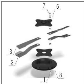
Corn blades – left + rotor cover
