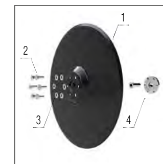
Drill coulter
