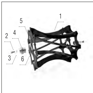
Slatted roller 350
