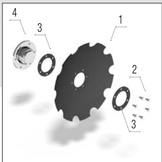
Serrated disc for the central unit 620 × 6 mm
