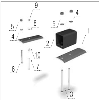
Front counter blades
