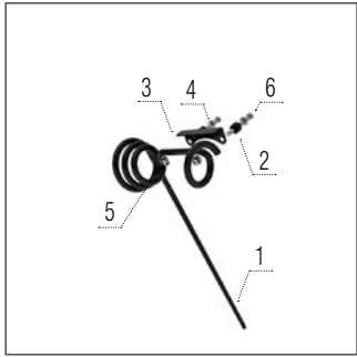
Three-row left harrow tine
