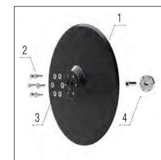
Drill coulter
