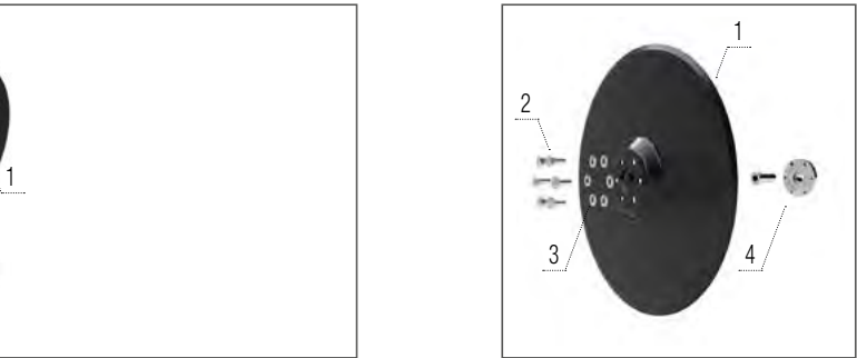
Depth wheel 330 × 65
