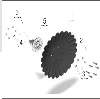
A-Disc 660 × 6 mm
