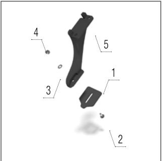
Abstreifer Cutpack
