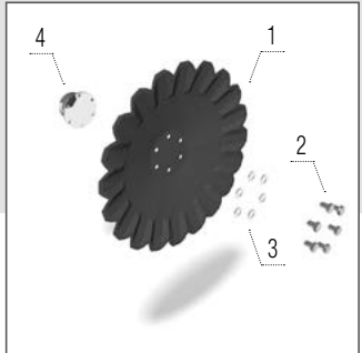
A-Disc 520 x 5 mm
