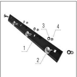
Trash Cutter 610
