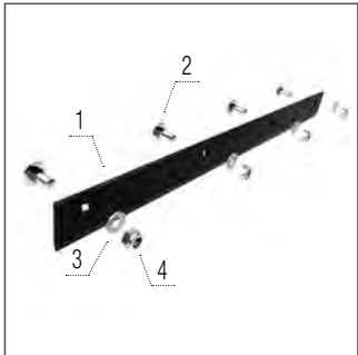
Trash Cutter 750
