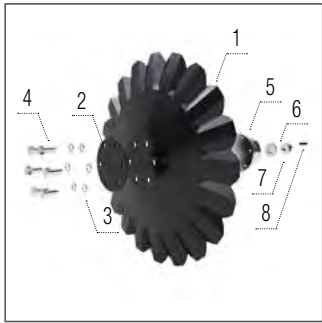
A-Disc 560 × 5 mm
