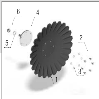
A-Disc 620 × 6 mm
