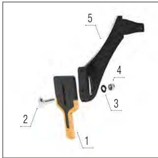
Abstreifer Hardface Cutpack
