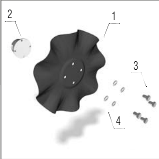
Coulter
