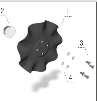
Coulter
