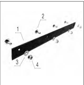
Trash Cutter 750
