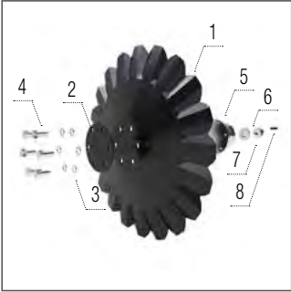
Disco A 560 × 5 mm
