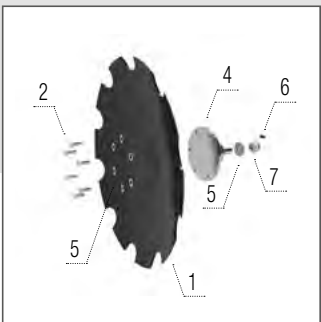
Disco A 620 × 6 mm
