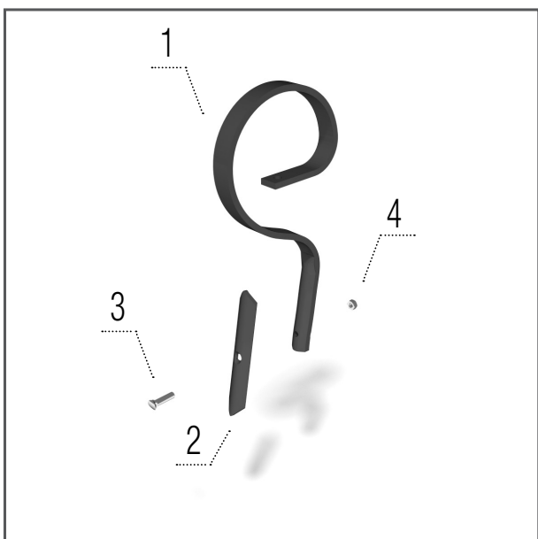
Gamma point
