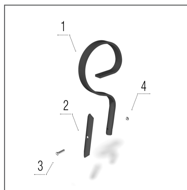
Gamma point
